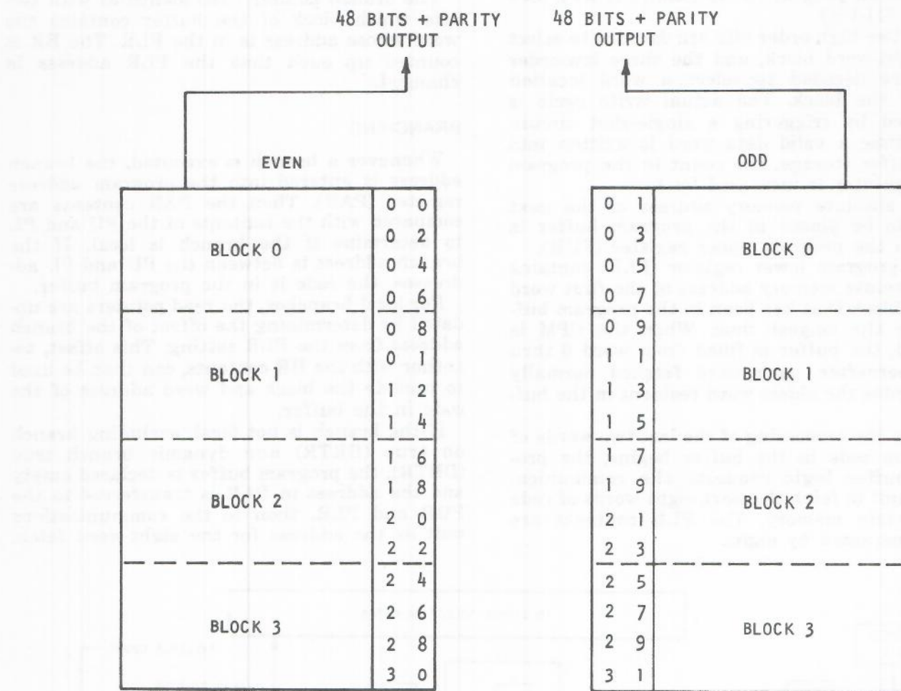
PROGRAM BUFFER FORMAT
