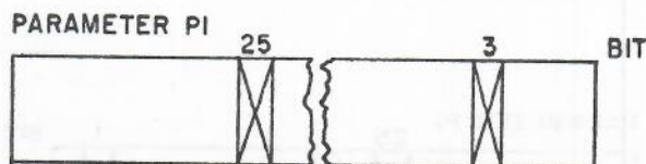
Invalid Address Interrupt Parameters
