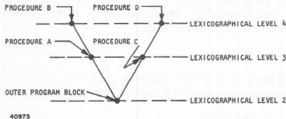
Figure II-2-8. Addressing Environment Tree of ALGOL Program
