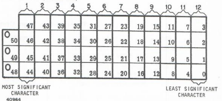
4-BIT DIGITS (PACKED BCD)
