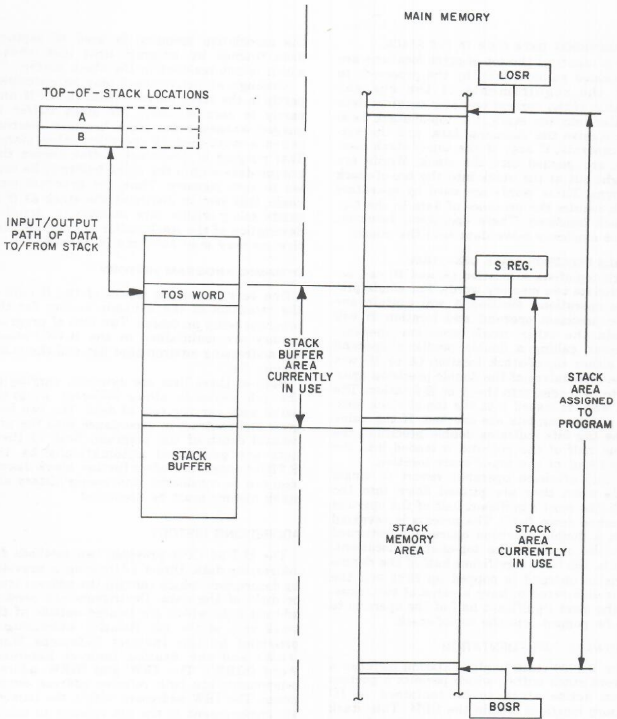
Figure II-2-5. Stack Buffer and Stack Memory Area
