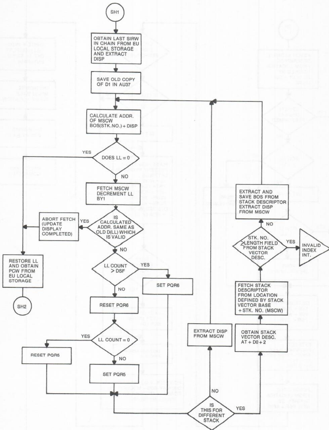
Figure III-3-8. Flow Chart of Enter Operator (Sheet 3 of 3)
