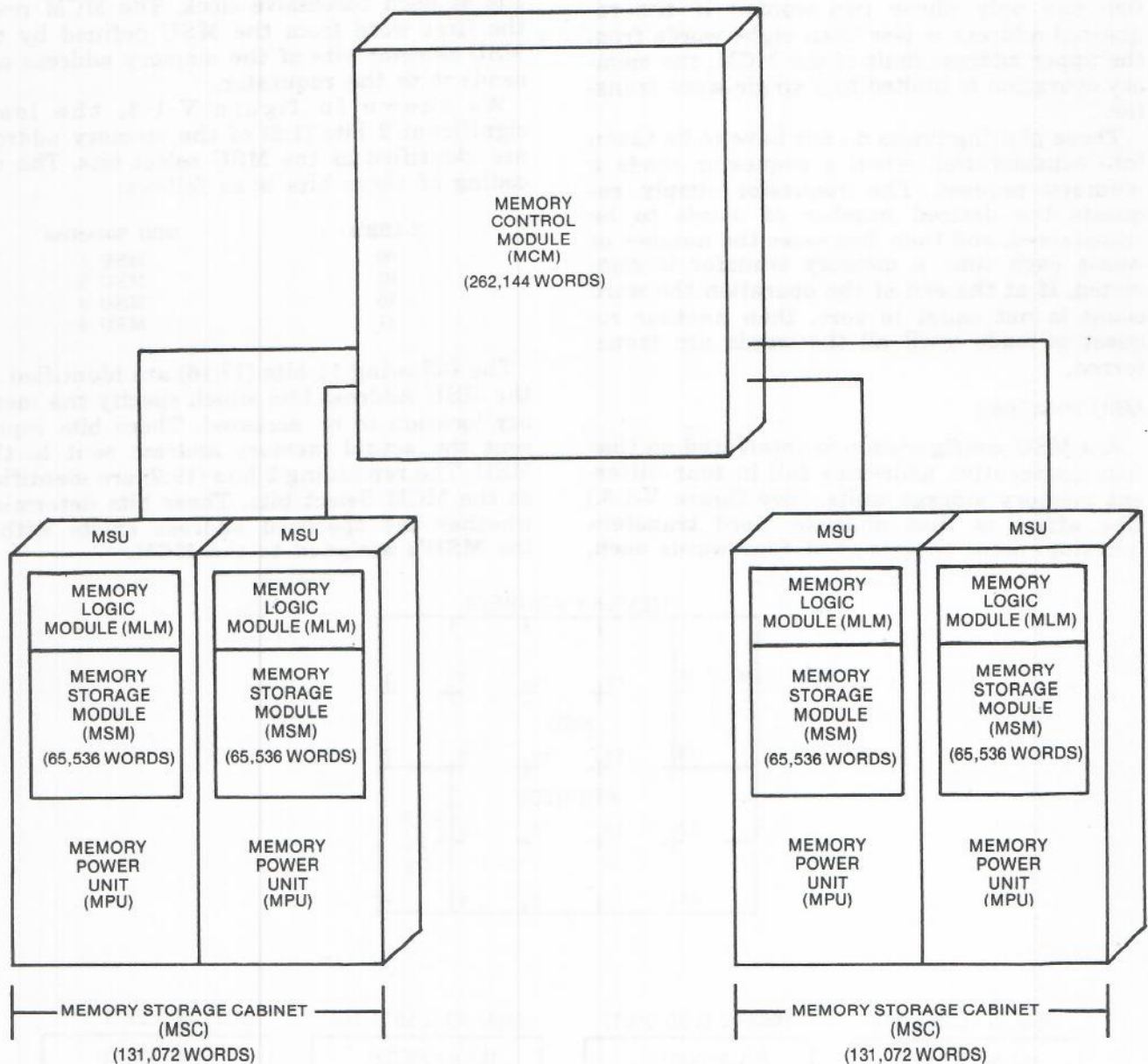
Figure V-1-2. B 7700 Memory Subsystem
