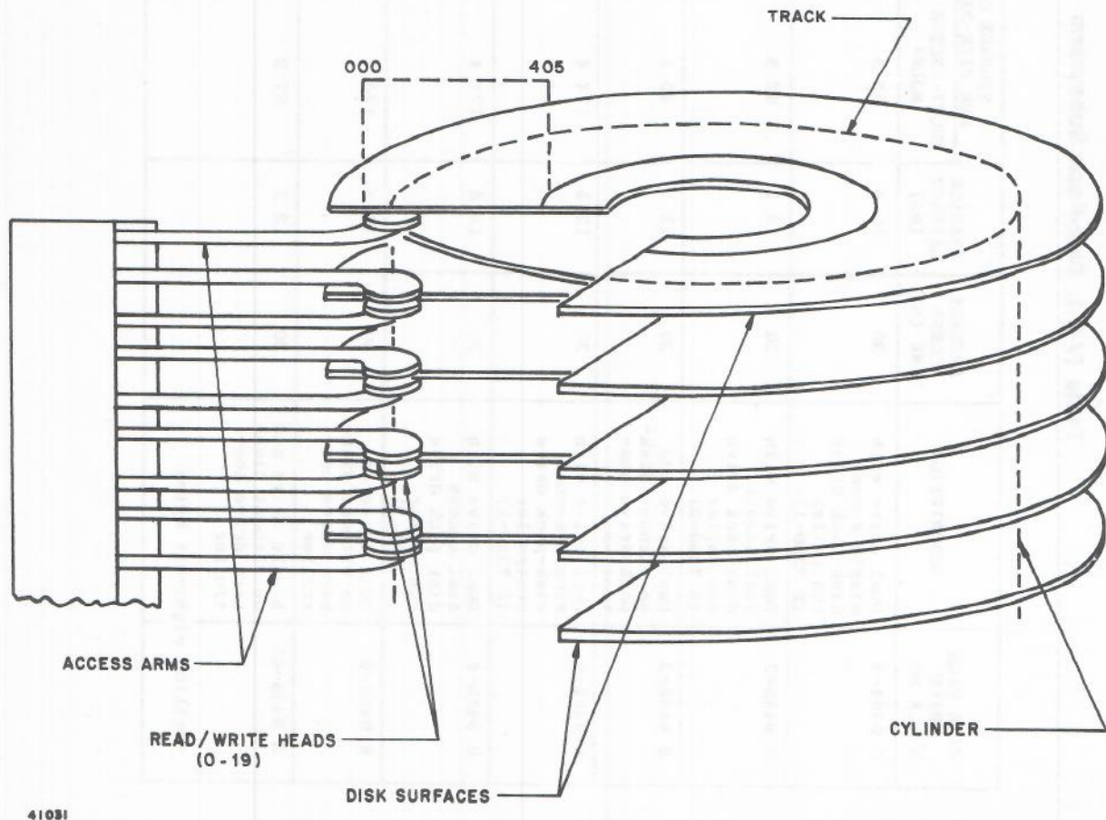
Figure IV-3-1. Disk-Pack Recording Surfaces
