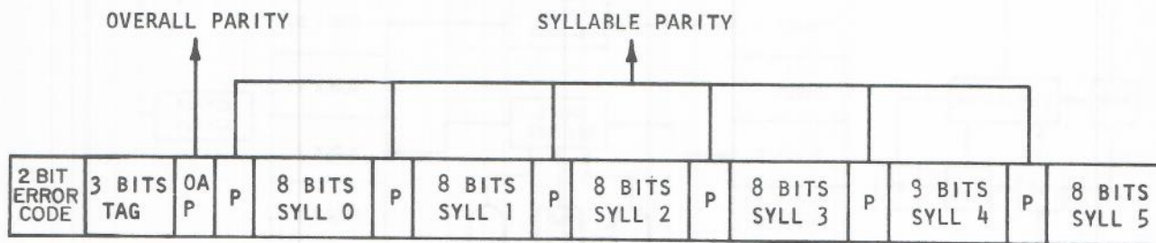
PROGRAM BUFFER WORD FORMAT
