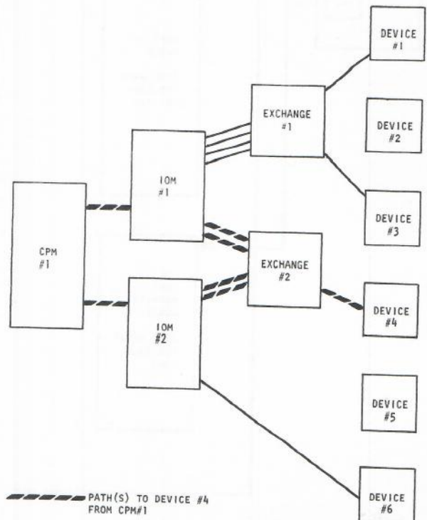
Figure II-4-2. Data Transfer Path Selection
