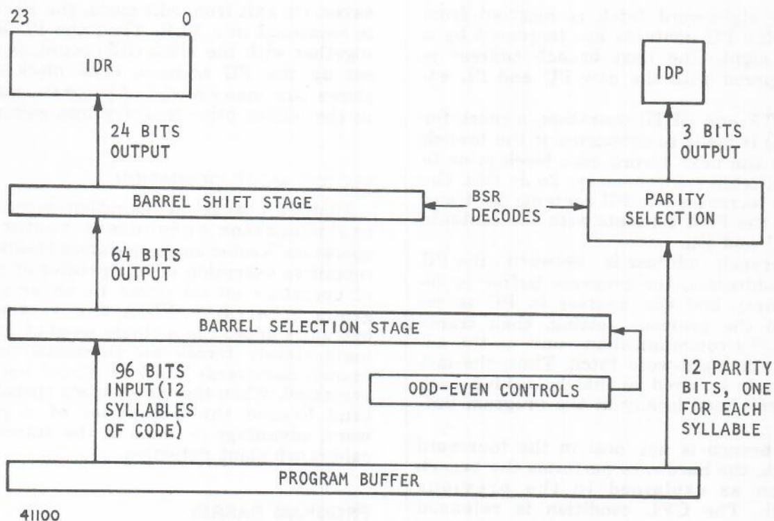
Figure III-1-6. Program Barrel
