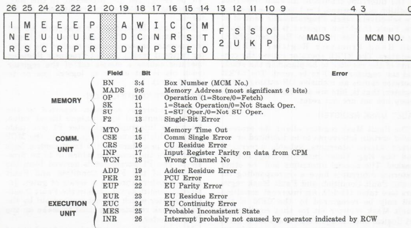
Figure III-2-1. CPM Fail Register
