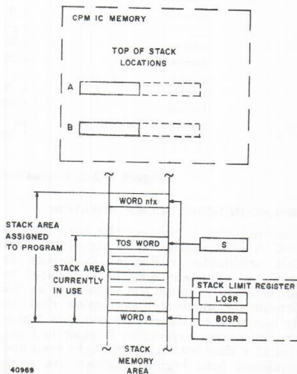
Figure II-2-4. Top of Stack and Stack Bounds Register
