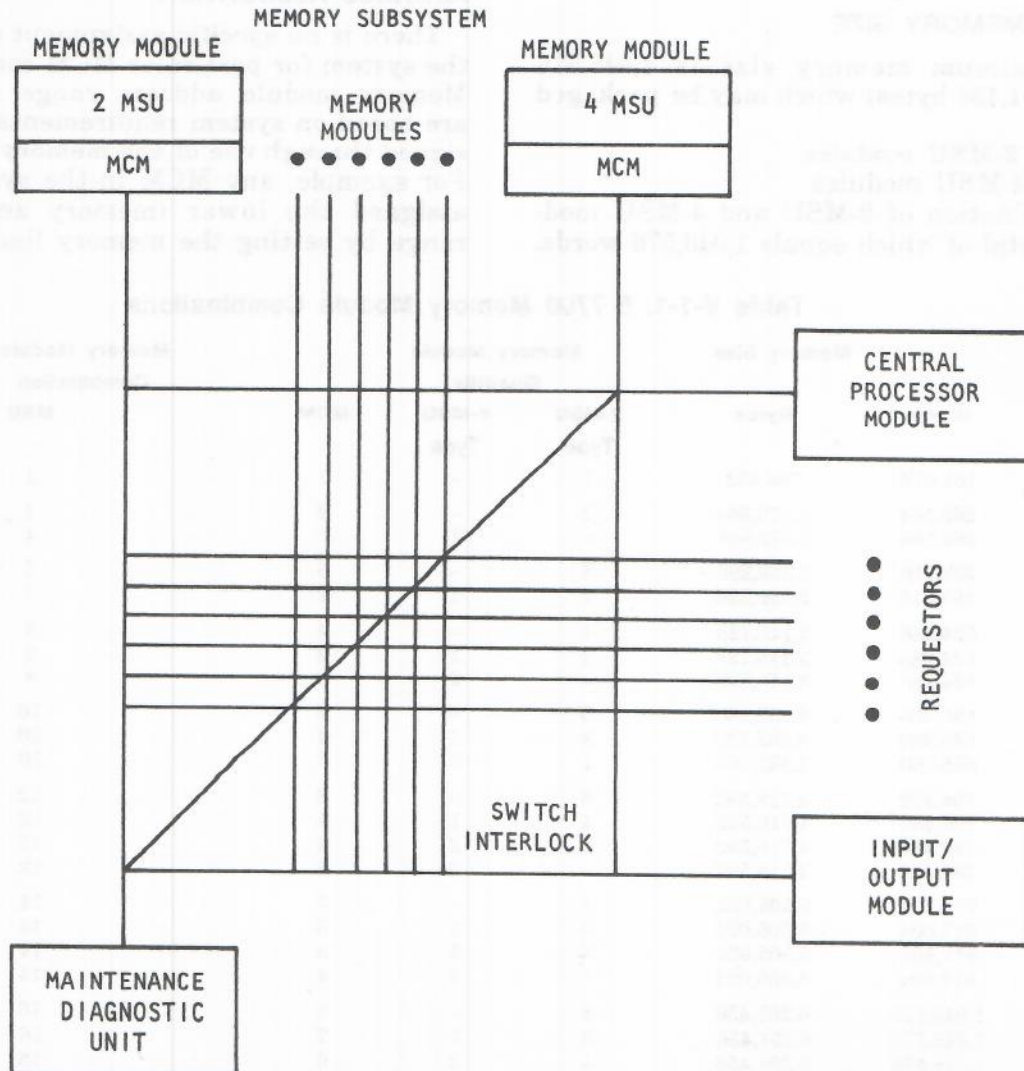
Figure V-1-1. B 7700 Memory System Modularity Diagram
