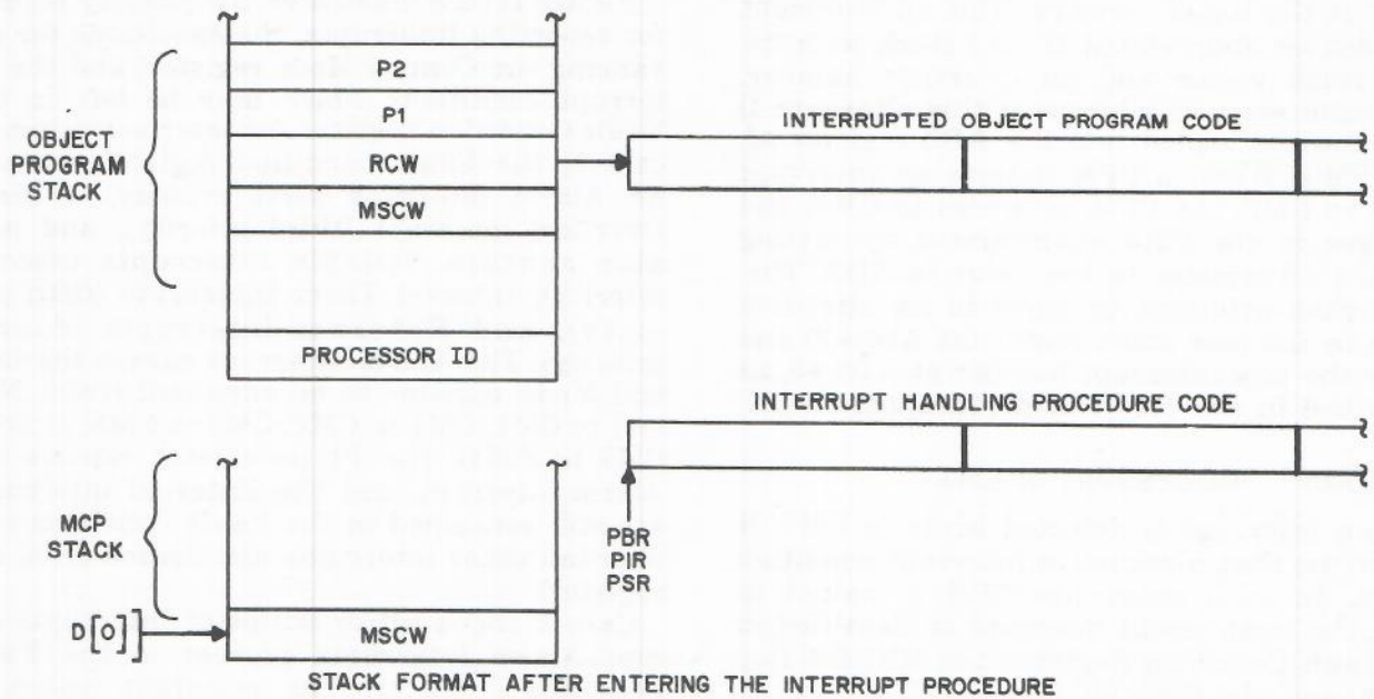
Figure III-2-3. Stack Format
