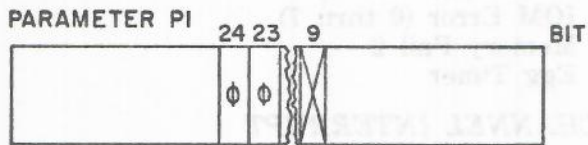
Sequence Error Interrupt Parameters
