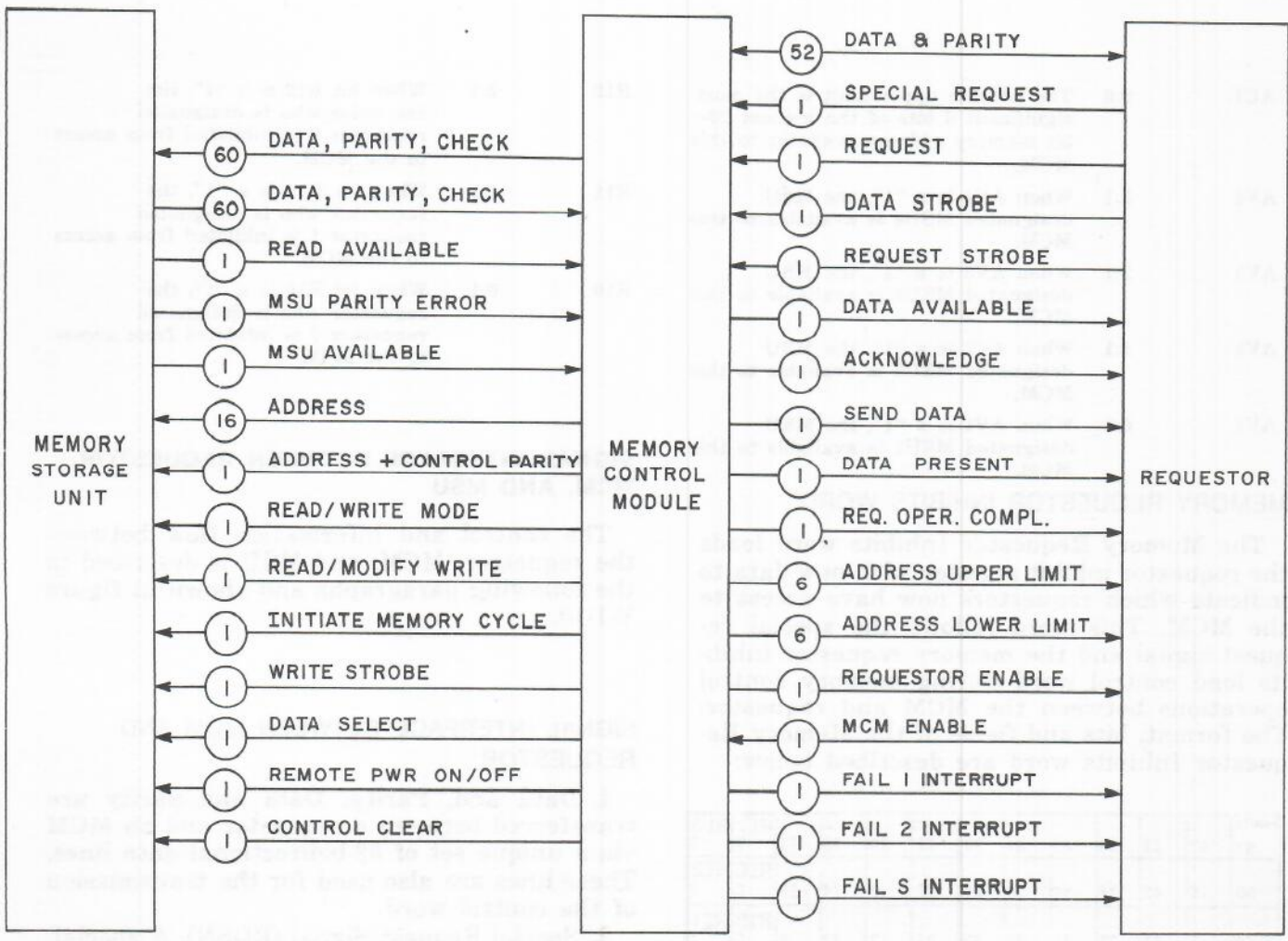
Figure V-1-10. Requestor-MCU-MSU Interface
