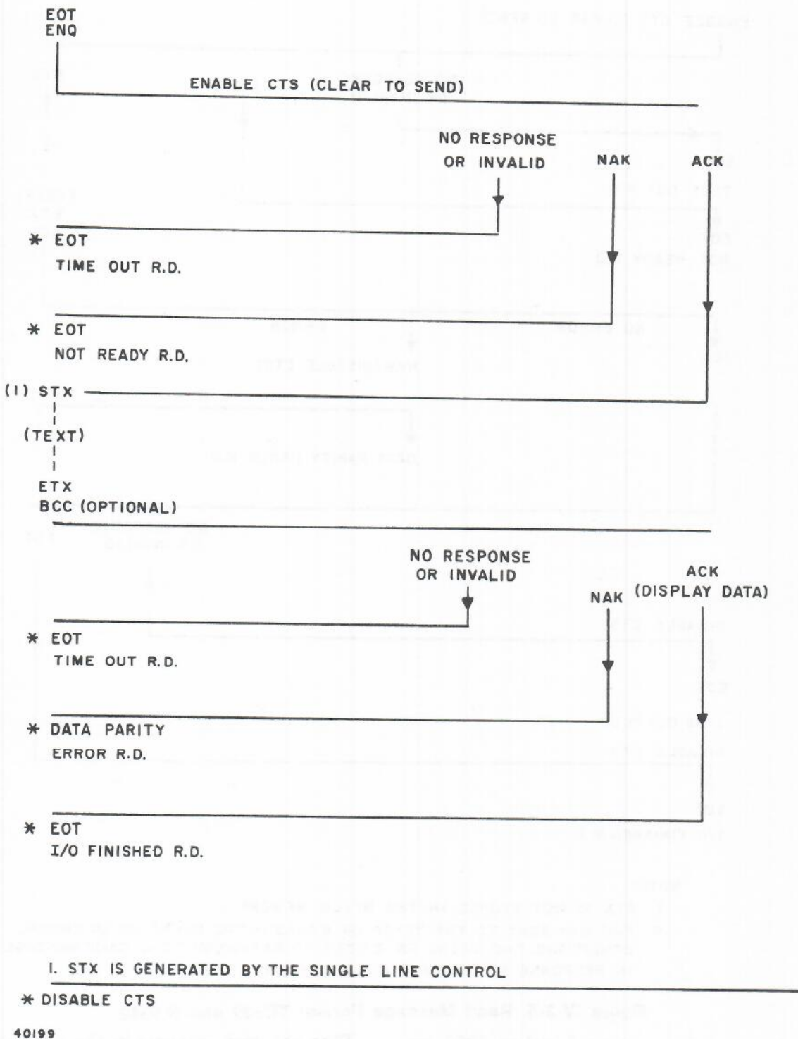
Figure IV-3-6. Write Message Format TC500 and B 9352
