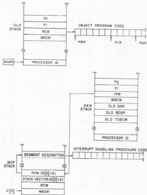
Figure III-2-4. Stack Format Prior to Calling Interrupt Procedure While in CM1 (Move Stack Operation)
