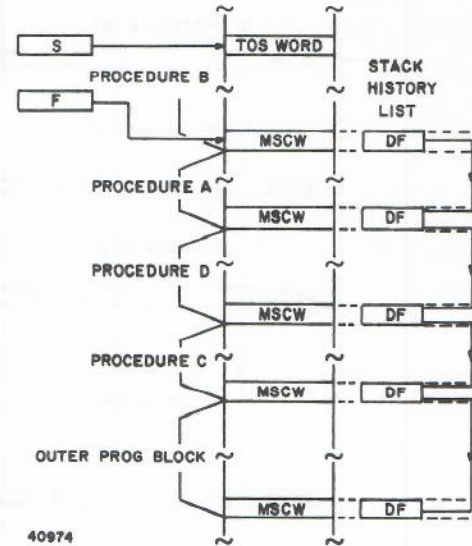
Figure II-2-9. Stack History List
