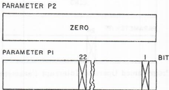
Stack Overflow Interrupt Parameters
