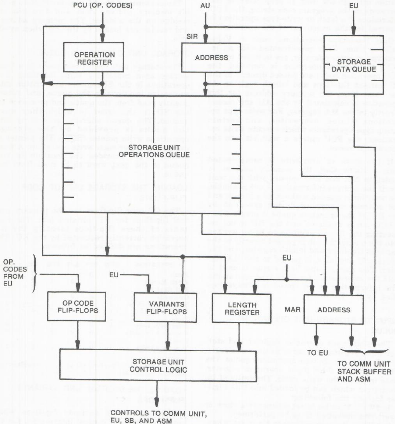
Figure III-1-15. Storage Unit
