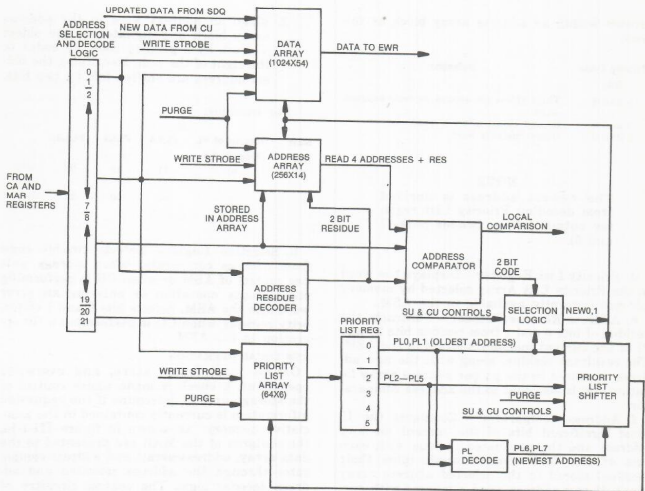
Figure III-1-14. Associative Memory
