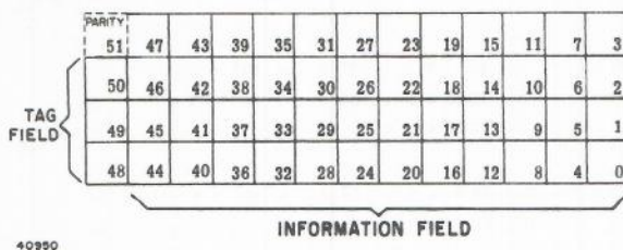
Figure II-1-1. Word Structure
