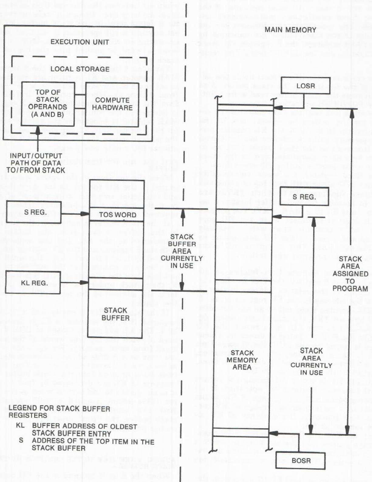
Figure III-1-12. Stack Buffer and Stack Memory Area
