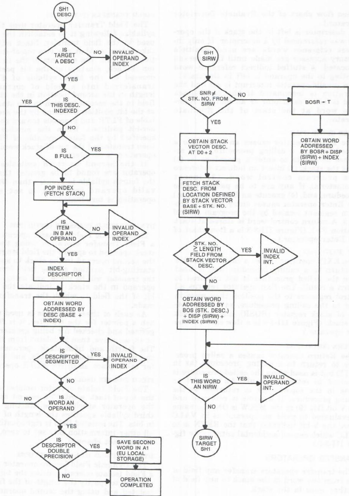
Figure III-3-6. Flow Chart of Value Call Operator (Sheet 2 of 2)
