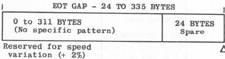
Figure IV-3-3. Single Sector For Track Format
