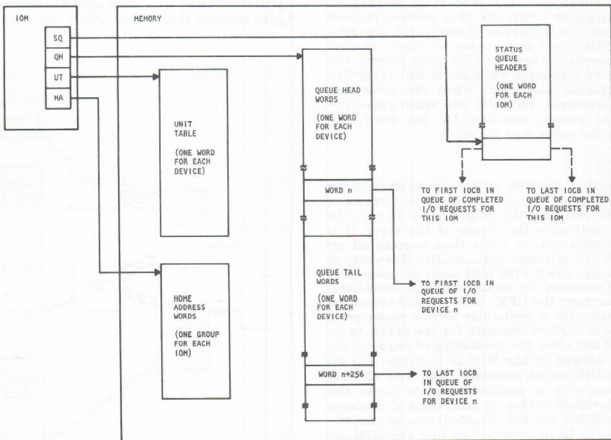
Figure II-4-3. I/O Subsystem Map, Simplified Block Diagram
