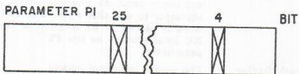
Stack Underflow Interrupt Parameters
