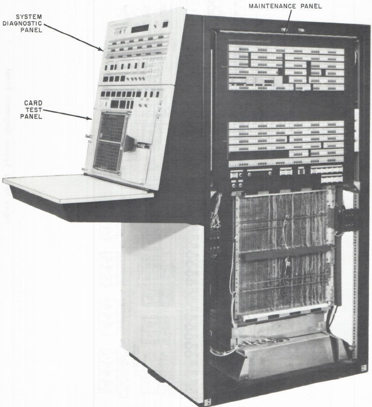
Figure VI-5-1. Maintenance Diagnostic Unit
