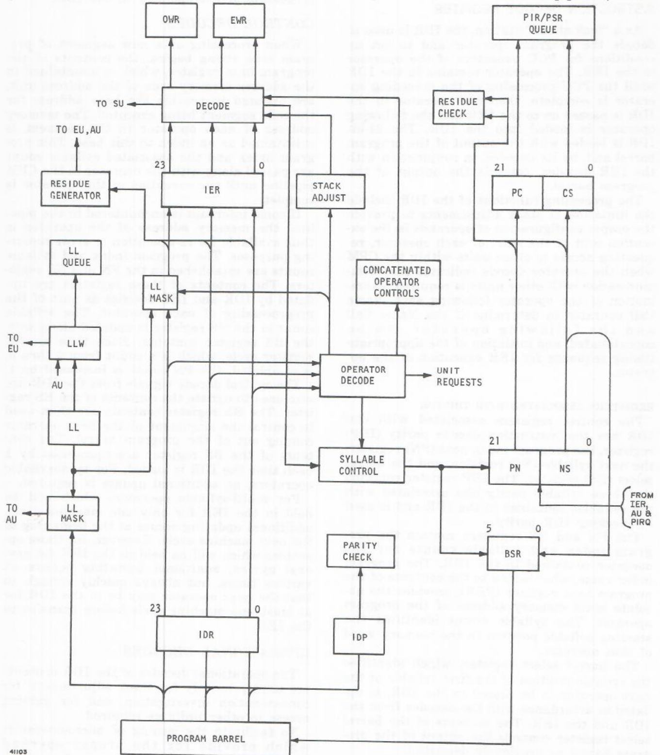
Figure III-1-7. Program Control Unit
