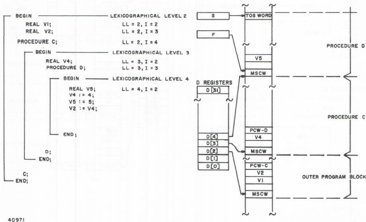
Figure II-2-6. ALGOL Program With Lexicographical Structure and Related Stack Structure
