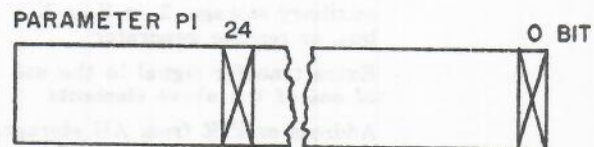
Memory Protect Interrupt Parameters
